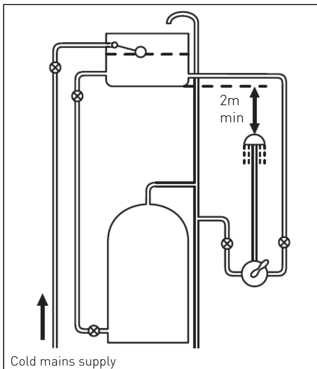
Gravity Fed Hot and Cold
